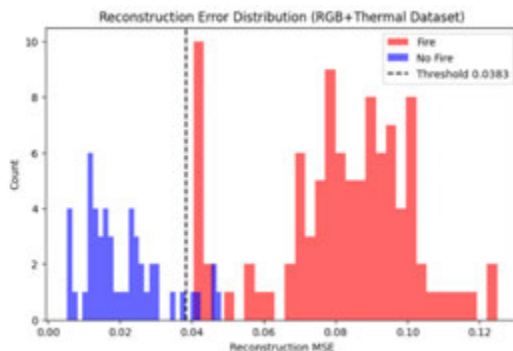
Figure 7 Reconstruction error distribution - Early fusion
