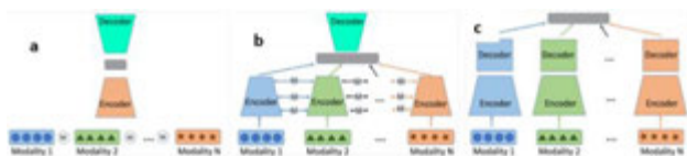
Figure 2 CAE based fusion approaches - a) Early - b) Feature level (mid-) c) Decision level (late-) fusion
