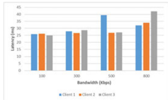
Figure 4 Impact of Bandwidth on latency
