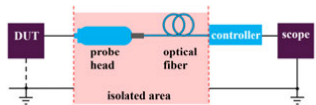
Figure 7 Isolating using optical fiber – illustration based on [8]
