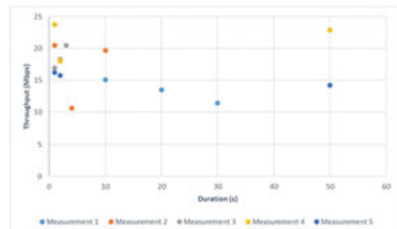
Figure 7 Impact of Transmission Duration on Throughput
