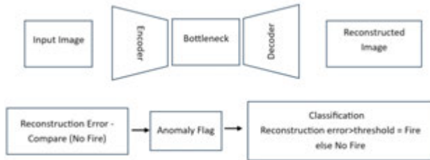
Figure 1 CAE based autoencoder algorithm to discriminate between Fire and No Fire
