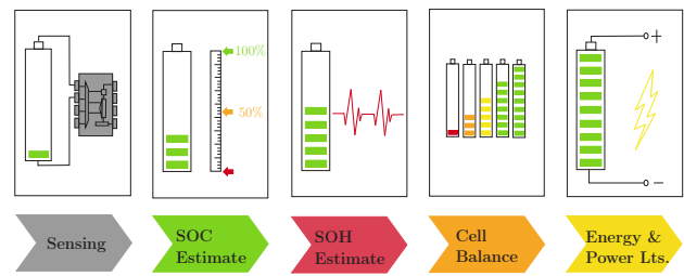
FIG 3. BMS Workflow [13]
