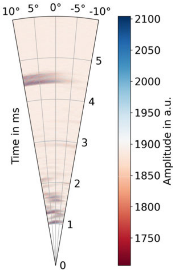
Figure 6: Line scan of an object placed 75 cm in front of the L-CMUT array at an angle of 5°.
