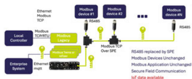
Figure 4 Adding IoT Connection
