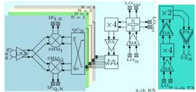
Figure 3 Block diagram of the J-band RX and TX ICs
