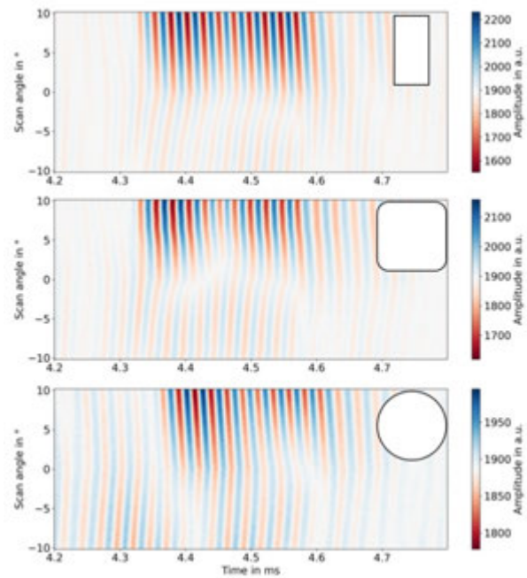
Figure 7: Reflection pattern of the scan of different object placed at 10° and 75 cm distance. Top: rectangular with sharp corners; Middle: rectangular with rounded corners; Bottom: circular.
