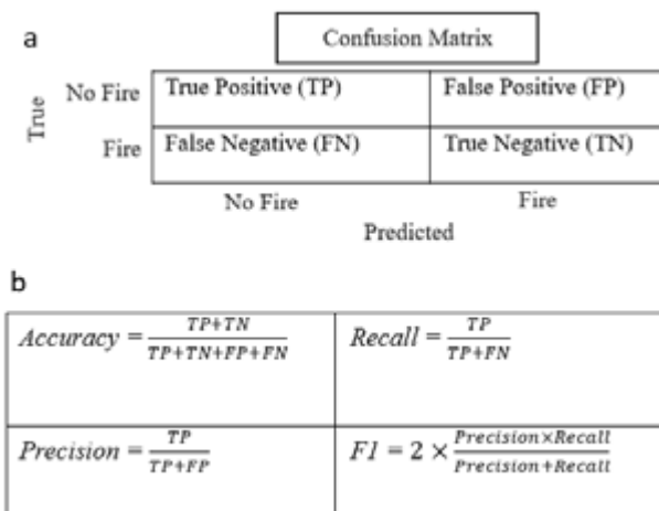
Figure 5 a) Confusion matrix b) Performance matrices derived from confusion matrix to evaluate the correctness of models
