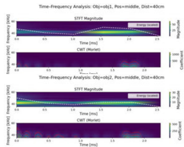
Figure 6. Time-frequency analysis of echoes at d = 40 cm, middle position. STFT magnitude spectrogram with overlaid normalized energy trace (white dashed line). CWT, with red contours indicating regions of high spectral energy.
