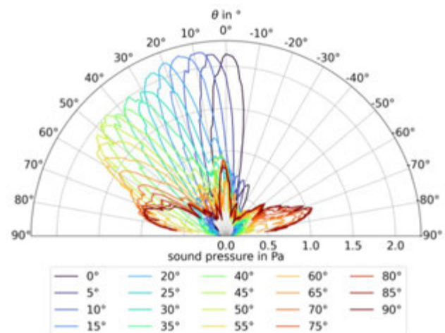
Figure 5: Measured sound pressures for different deflection angles.
