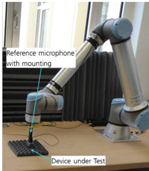
Figure 4: Actual measurement setup on the cobot.
