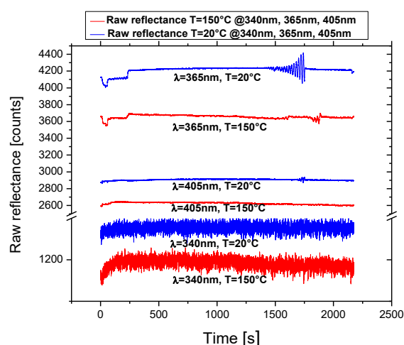
Figure 2 Raw data of etching transients recorded at different etching temperatures on samples from the same epitaxial run.
