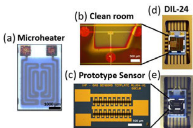
Figure 1 (a) Microheater, (b) \text{CeO}_2/\text{SnO}_2 -based sensor chiplet, (c) \text{SnO}_2 -based sensor chiplet, (d and e) sensor chiplets integrated with microheater and wire-bonded to a DIL-24 socket.
