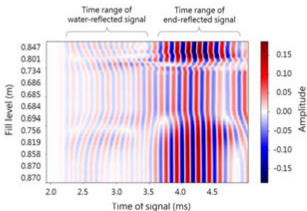
Figure 3: Time domain heatmap of measured guided wave signals showing the time ranges of the water reflection and the end reflection for varying liquid fill levels.
