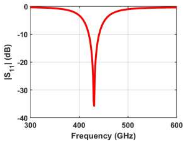
Figure 6 Reflection coefficient ( S_{11} in dB)
