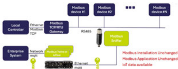
Figure 2 IoT Add On Data Sniffer
