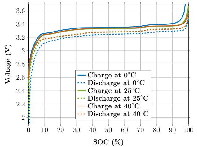
FIG 5. OCV vs SOC curves [20]
