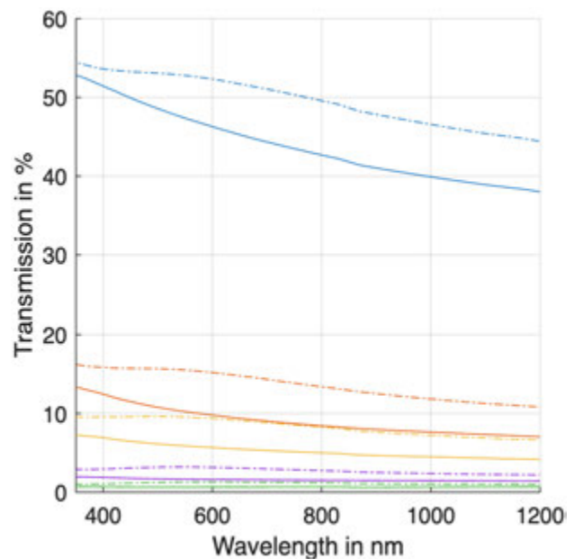
Fig. 2 Transmission of Palladium on Float Glass at 0 % (solid line) and 5 % v/v hydrogen in Ar (dash-dotted line) over the wavelength in nm for various thicknesses of Pd: 15 nm (blue), 22 nm (orange), 30 nm (yellow), 45 nm (purple), 60 nm (green).
