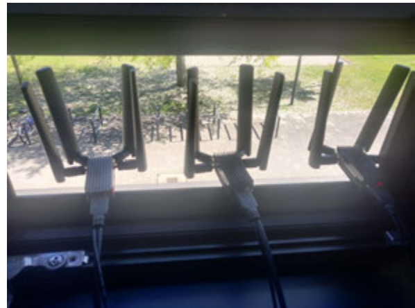
Figure 2 Client 5G dongles setup
