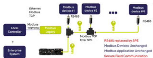
Figure 3 Switching from RS485 to SPE
