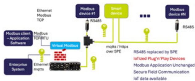
Figure 6 Changing to IoT Communication
