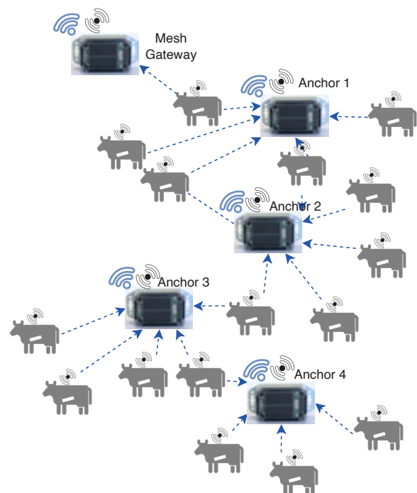
Figure 1 Architecture of a solar-power mesh network with bolus inside the cows roaming in the farm in between the mesh nodes (Anchors)
