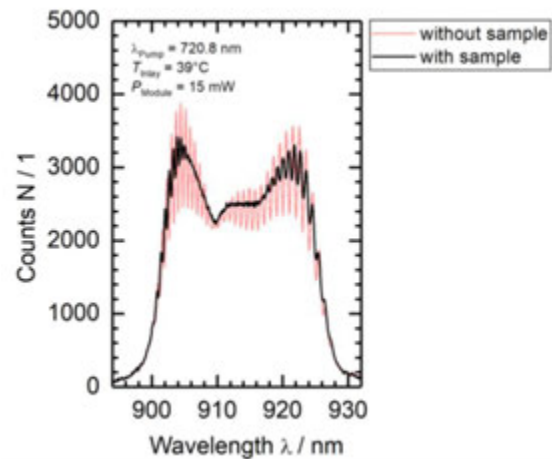
Figure 6 NIR spectrum with and without polymer sample placement in the idler arm.
