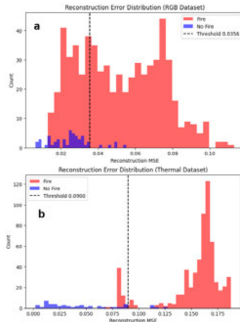
Figure 6 Reconstruction error distribution a) RGB dataset b) Thermal dataset
