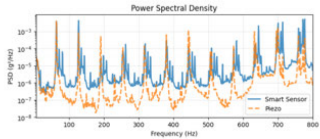
Figure 3: Power spectral density of piezo (orange) and smart sensor (blue) during milling process
