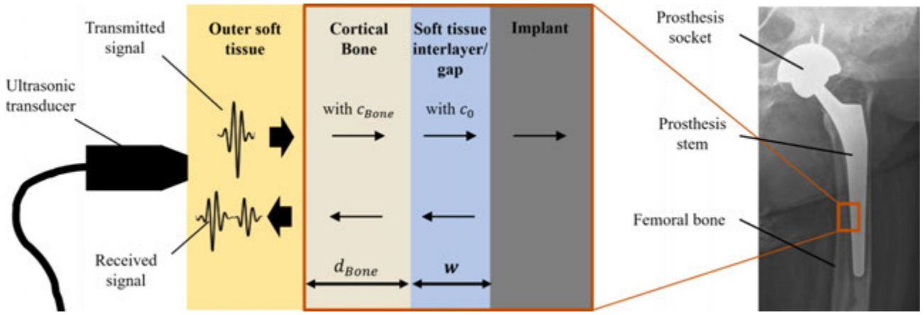
Figure 1 Multilayer model of the thigh with hip prosthesis stem.
