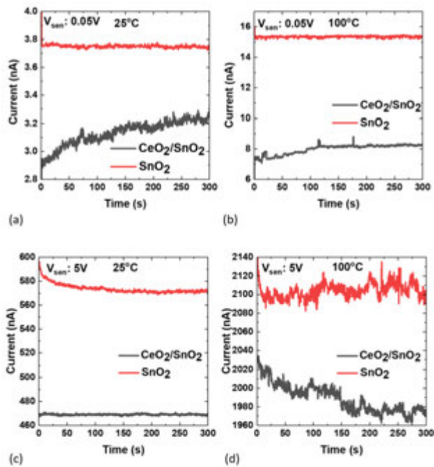
Figure 3 Observations of current drift in the CeO 2 /SnO 2 channel (black) and the SnO 2 -only channel (red) at low voltage (a and b) and high voltage (c and d) at room temperature and 100°C, respectively.
