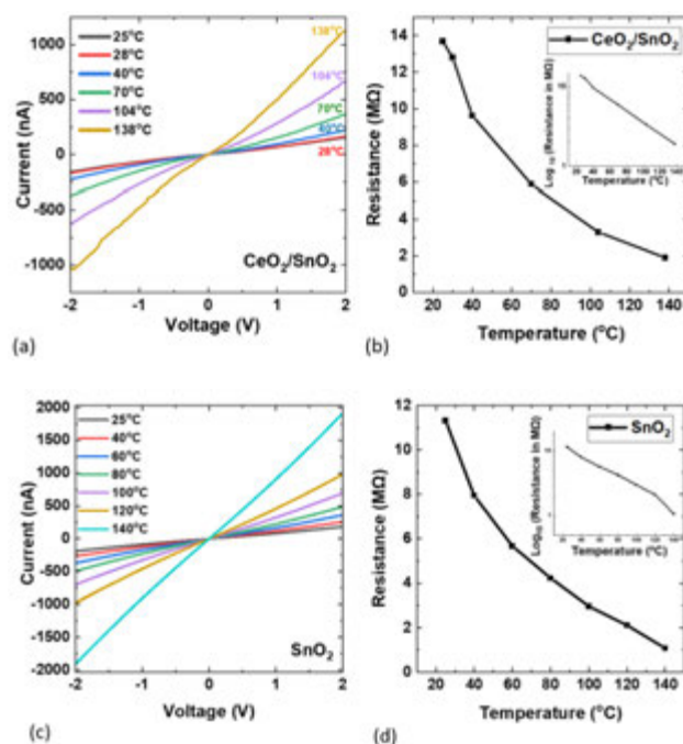
Figure 2 Effects of temperature on both \text{CeO}_2/\text{SnO}_2 and \text{SnO}_2 -only structures. I-V characteristics with heating (a) \text{CeO}_2/\text{SnO}_2 (micro-heater voltage) and (c) \text{SnO}_2 . (b and d) Resistance variation with temperature increase in \text{CeO}_2/\text{SnO}_2 and \text{SnO}_2 -only structures, respectively. Inset: log (resistance) vs. temperature.
