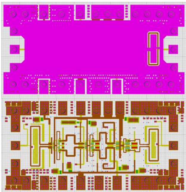
Figure 2 Layout of InP PA, top layer (top) and layer below top (bottom).
