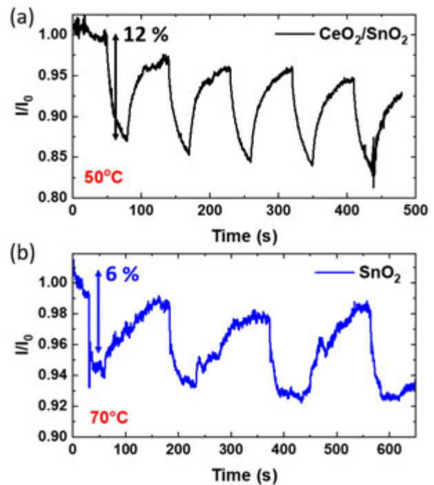
Figure 4 Current variation upon exposure to 1% H 2 /air gas mixture at different temperatures in (a) CeO 2 /SnO 2 sample and (b) SnO 2 -only sample.
