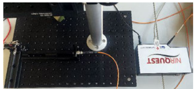
Figure 1 The view on the laboratory set-up used for experimentation.
