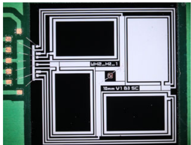
Fig. 1 Final sensor chip with four photodiodes and LED, mounted and bonded, chip size is approx. 12.6 x 12.6 mm 2
